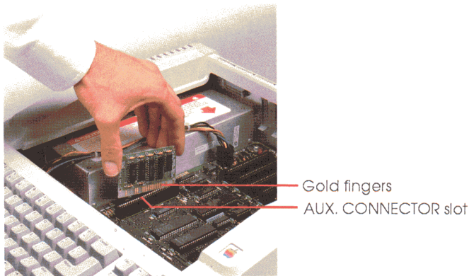
Figure 1-6 Removing the Extended 80-Column Text Card
