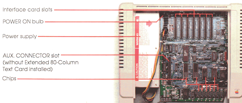
Figure 1-5 The Apple IIe main logic board
