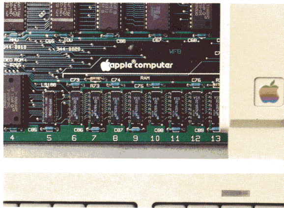
Figure 4-3 RAM chips
