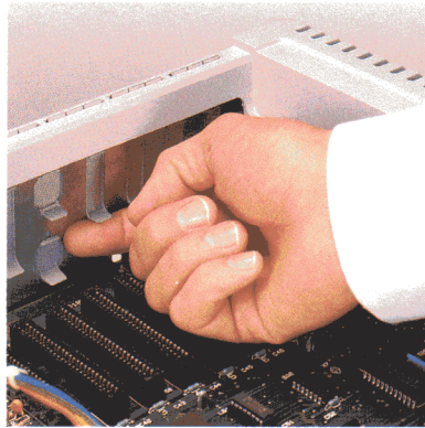
Removing a plastic insert
