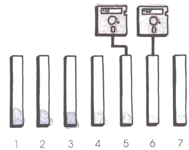
Figure 1-8 Suggested slots for two controller cards
