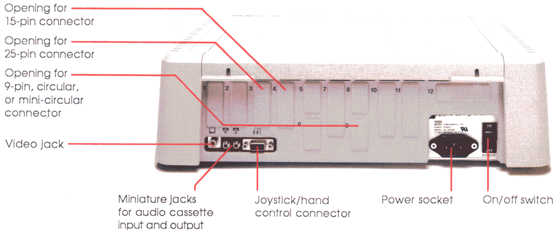
Figure 1-11 Back panel of the Apple IIe
