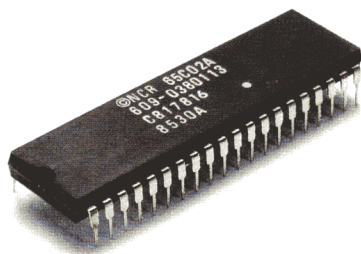
Figure 4-2 The microprocessor
