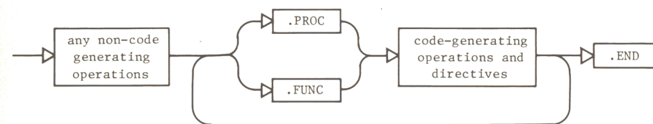
ASSEMBLY-FILE SYNTAX
