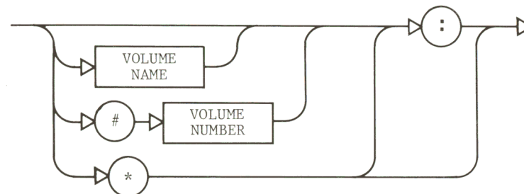
VOLUME-SPECIFICATION SYNTAX
