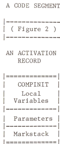
Figure 6 Detail of the "COMPINIT" Activation Record
