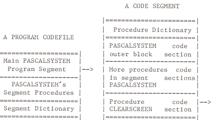
Figure 1 Complete Codefile of "The Program"
