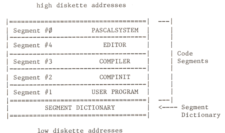
FIGURE 1 COMPLETE CODEFILE OF "THE PROGRAM"
