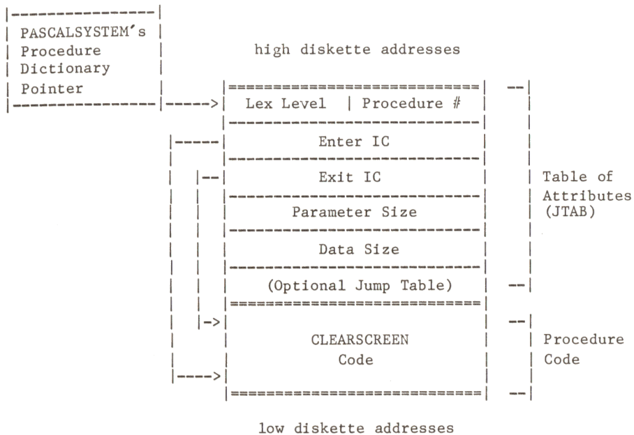
FIGURE 3 DETAIL OF THE "CLEARSCREEN" PROCEDURE CODE SECTION
