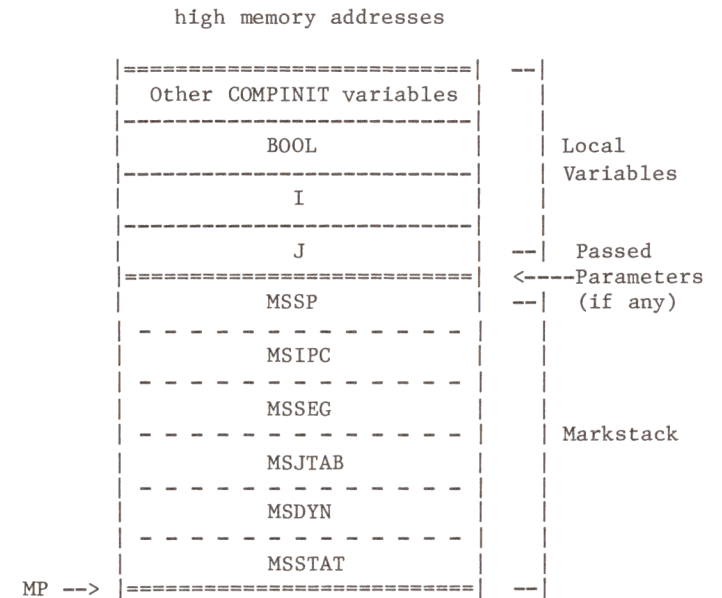
FIGURE 6 DETAIL OF THE "COMPINIT" ACTIVATION RECORD
