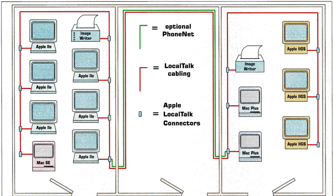
Figure 1. Sample AppleTalk network — bus configuration.
