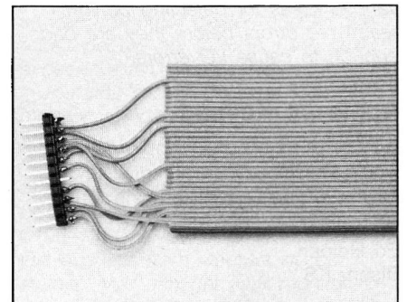
Photo. Adapter for connecting an Apple //e keypad to an Apple //c.
