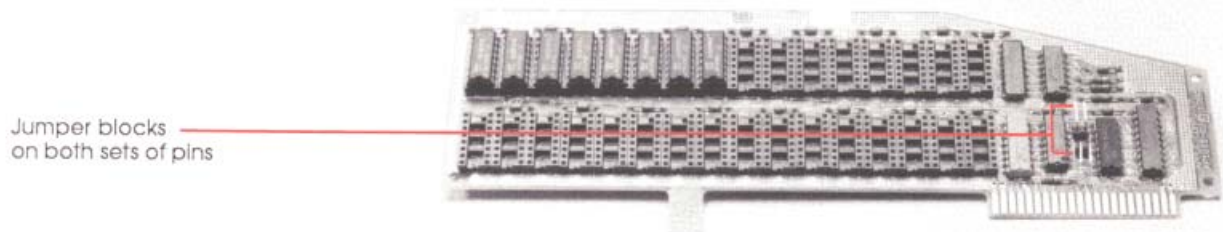
Figure 3-2 1-megabyte upgrade
