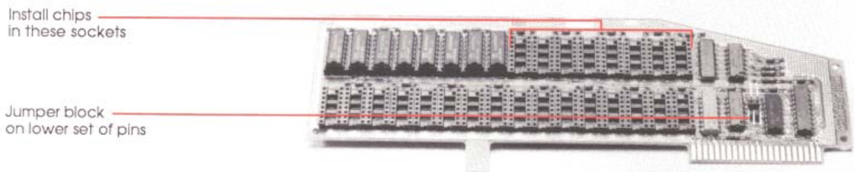
Figure 3-1 512K upgrade
