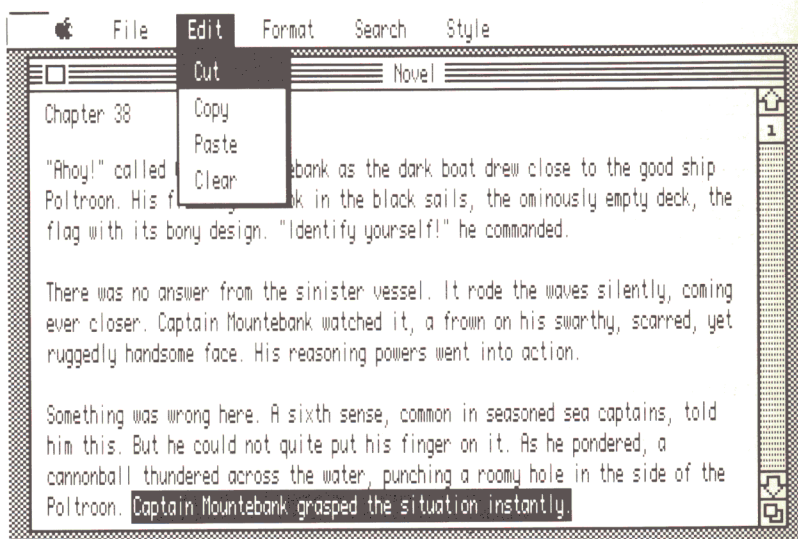
Figure 4-9 Cutting text
