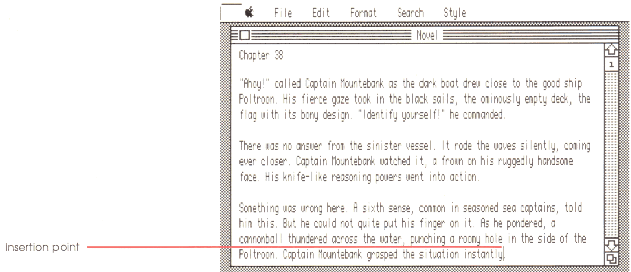
Figure 4-6 Insertion point
