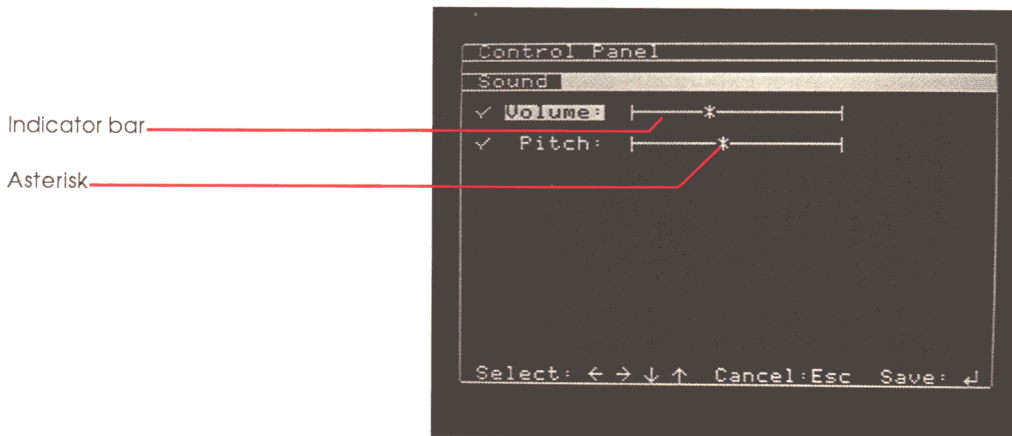
Figure 3-7 Changing volume
