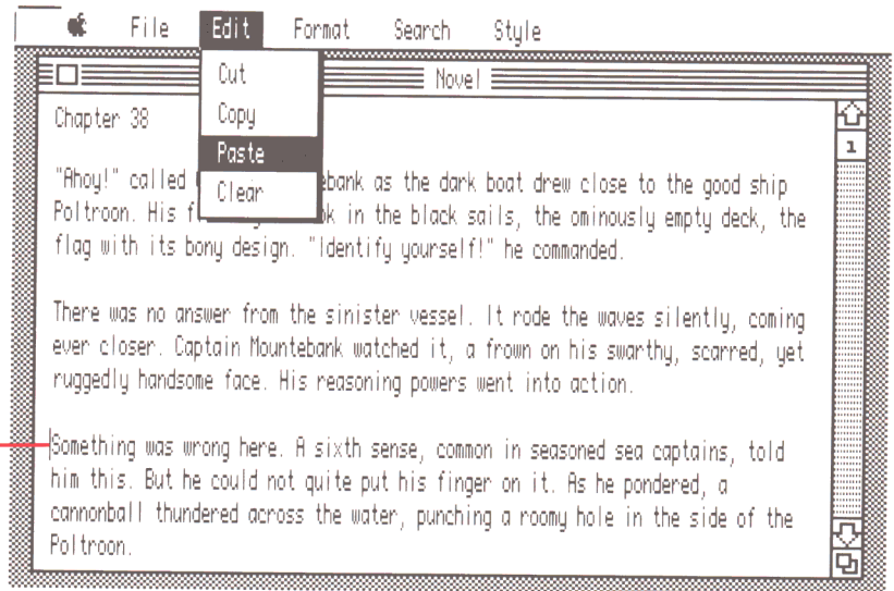
Figure 4-10 Pasting text
