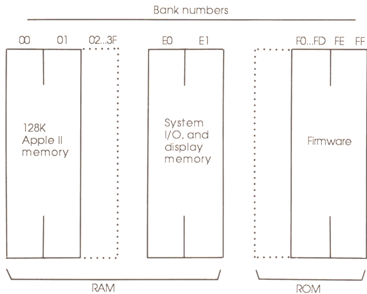
Figure B-1 Memory map
