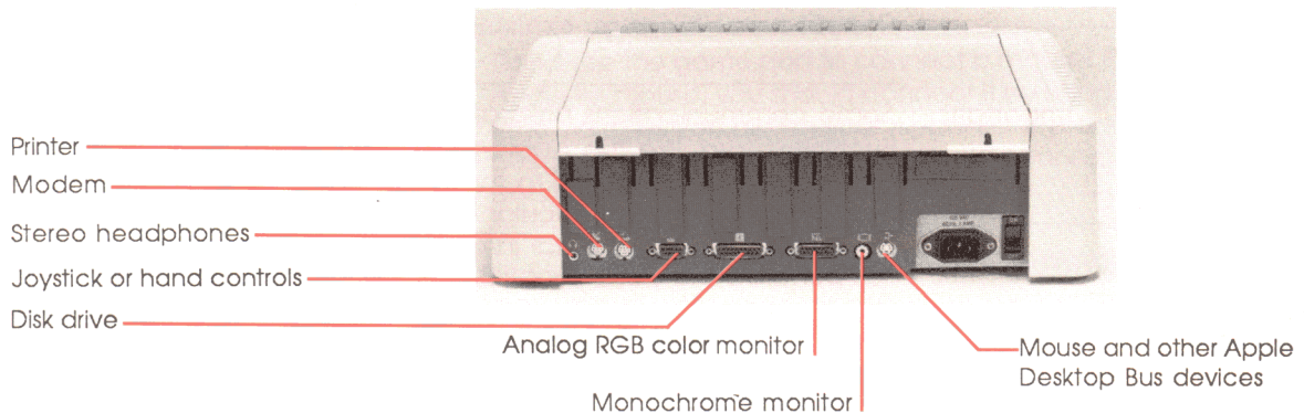
Figure 2-2 Ports
