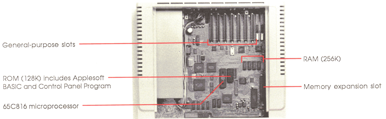
Figure 1-1 Main circuit board
