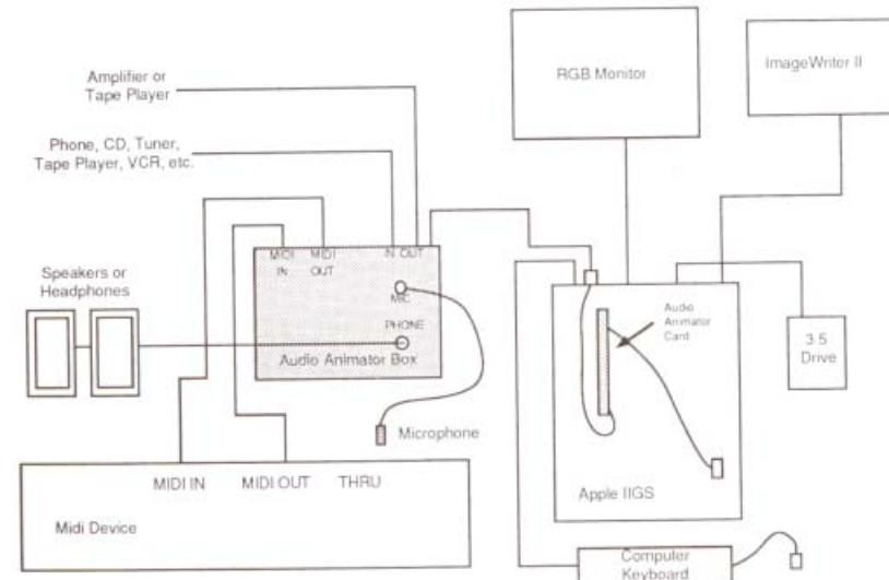
Typical Setup
