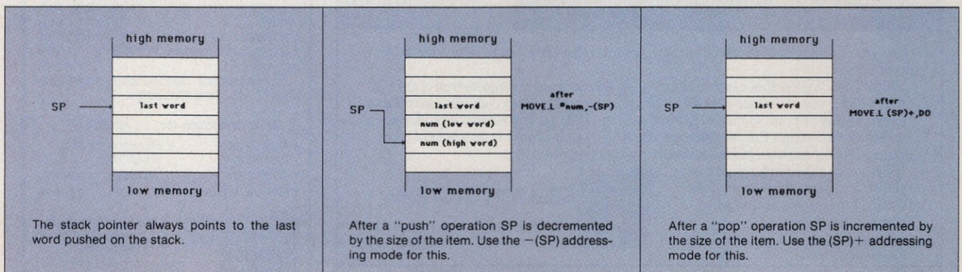
Figure 3: The 68000 stack and stack pointer. The address at the top of the stack is stored in the current stack-pointer register, SP.
