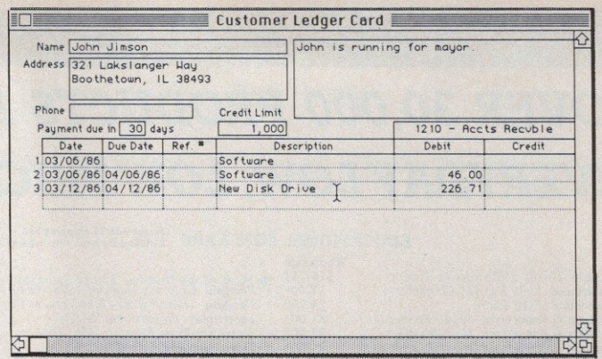
Figure 2: A customer ledger card from Plains & Simple
