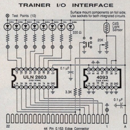
Figure 3: With a little work, you can produce drawings as complex as circuit diagrams.
