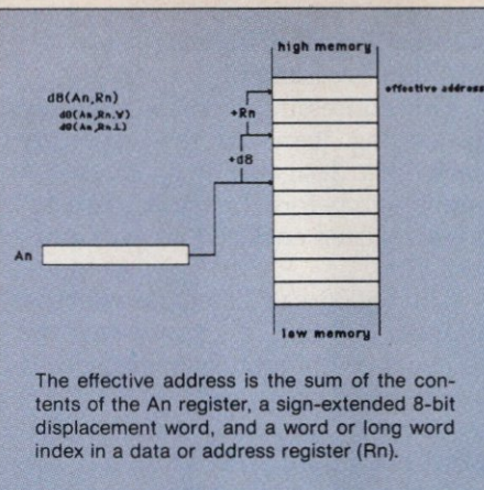
Figure 2: Address Register Indirect with Index addressing mode
