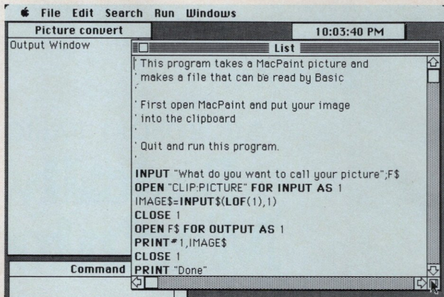
Figure 1: The MS-BASIC 2.1 programming screen. The List window is currently active, and the clock is the usual desktop accessory.
