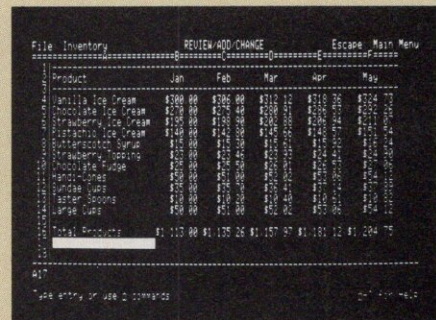
Figure 4: Inventory worksheet
