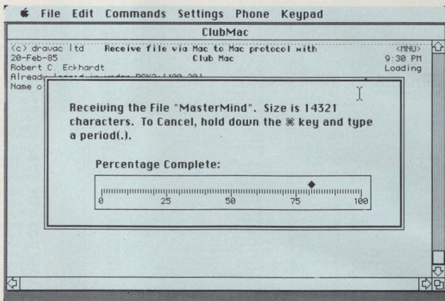
Figure 1: When you download files from the Club Mac BBS using MacTerminal and VT-100 emulation, a ruler-like meter shows you how the transfer is progressing.
