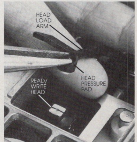
Figure 10: You can easily replace the head-pressure pad by squeezing the clip and pulling the head-load pad out of its holder.
