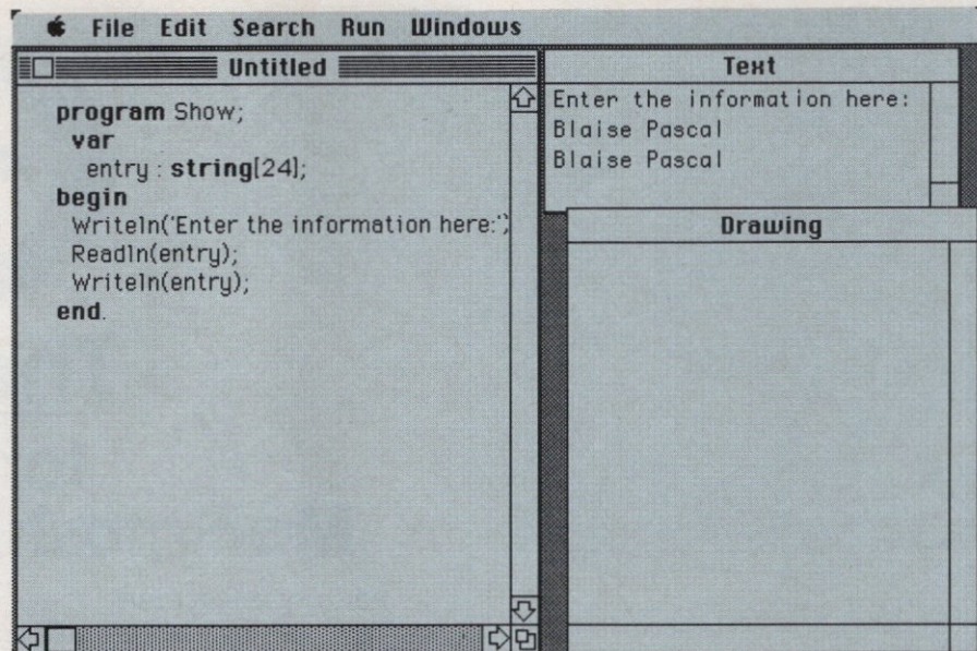
Figure 14: The screen after entry of a first and last name—the entire name must have 24 or fewer characters.
