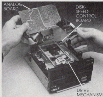
Figure 1: The main interior components of the disk drive
