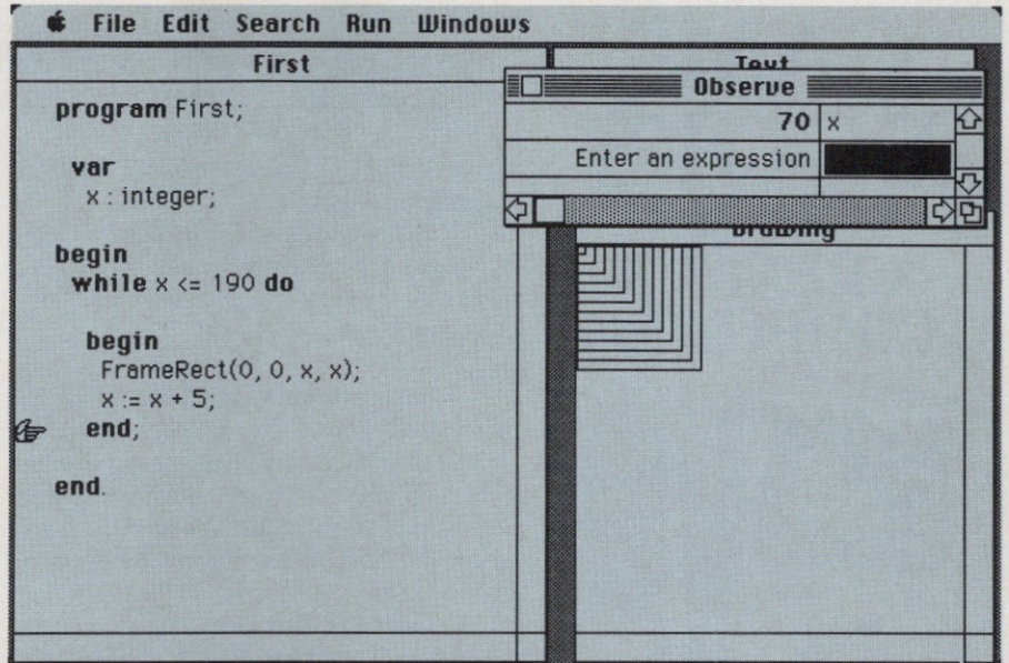
Figure 10: The screen looks like this after you hold down the ⌘ and S keys.
