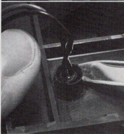
Figure 6: You can correct the position of the write-protect switch by adjusting the screws that hold it in place. When removing the front panel, make sure you disconnect the IN USE light first.
