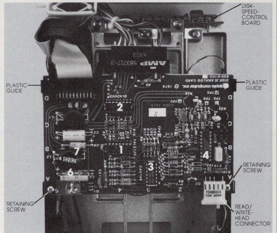
Figure 4: Analog-card components (in order of their frequency of failure): 1. 74LS125 (the drive-control circuit) 2. ULN2003 (stepper-motor drivers) 3. 3146 (write/erase transistor array) 4. 3470 (read and bias amplifier) 5. IC sockets (holds integrated/circuit chip, underneath number 1, 2, 3 and 4) 6. C4 (filter capacitor) 7. C5 (filter capacitor)
