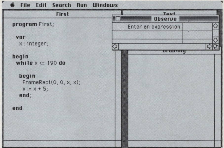
Figure 7: The First program—note the variable declaration under var.
