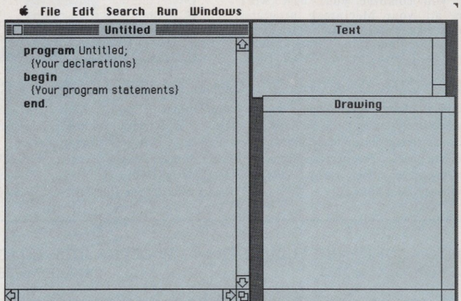
Figure 1: You'll see the Macintosh Pascal desktop when you get started.
