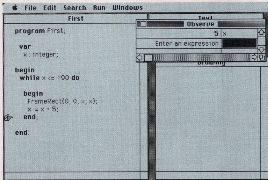
Figure 9: The desktop after you've single-stepped through the First program
