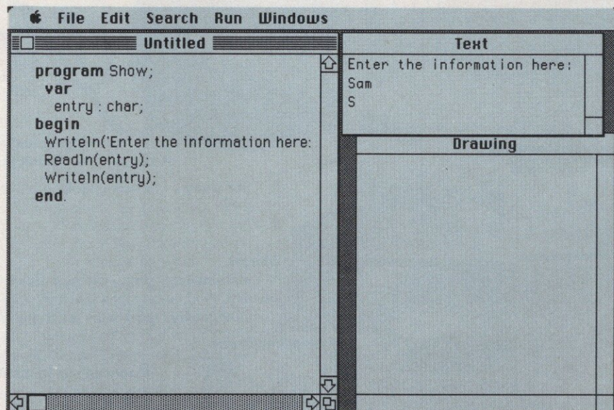
Figure 13: The screen after you've checked the program and typed Sam
