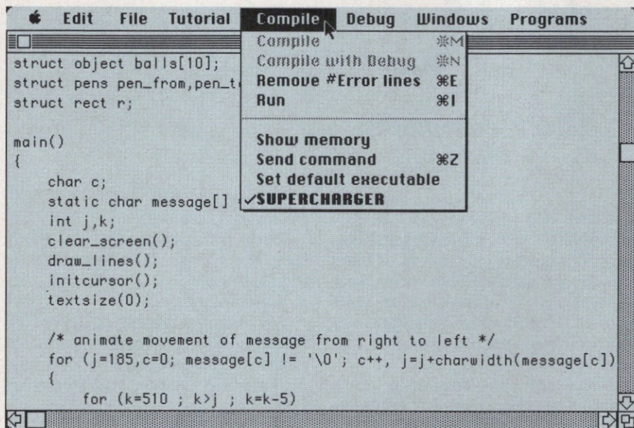
Figure 2: Hippo-C with the Compile menu pulled down
