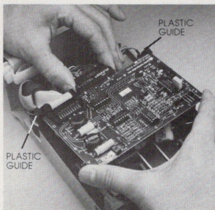
Figures 2 and 3: Removing the analog board: Unplug the read/write-head connector, unscrew the front retaining screws, and slide the board forward until it clears the plastic guides in the back.
