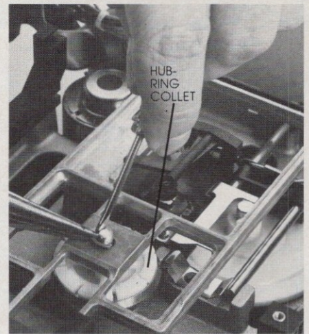
Figure 8: To replace the hub-ring collet or spring, remove the C ring, using a screwdriver and needle-nose pliers.
