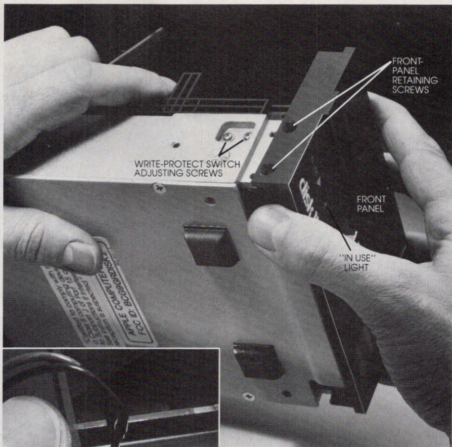
Figure 6: You can correct the position of the write-protect switch by adjusting the screws that hold it in place. When removing the front panel, make sure you disconnect the IN USE light first.
