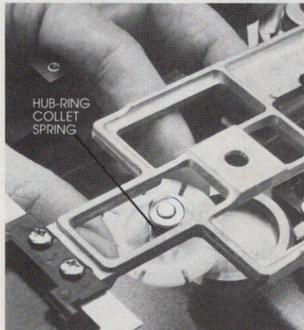
Figure 9: The hub-ring collet clamps the diskette down when the disk-drive door is closed. If the ring does not clamp down securely, look for a weak clamping action due to a defective spring.
