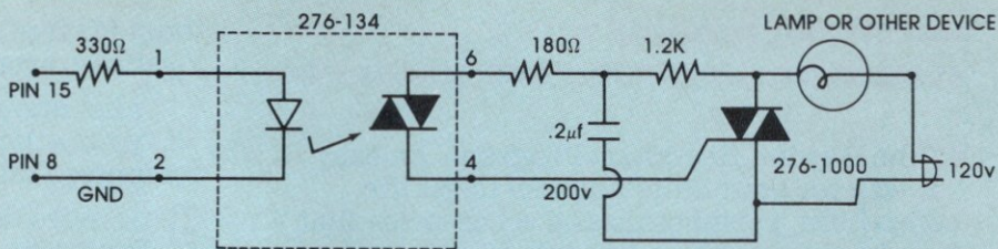
Figure 4: You can control appliances directly by connecting an optocoupler with a triac output.
