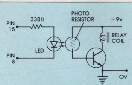
Figure 3: Complete electrical isolation with an opto-isolation system
