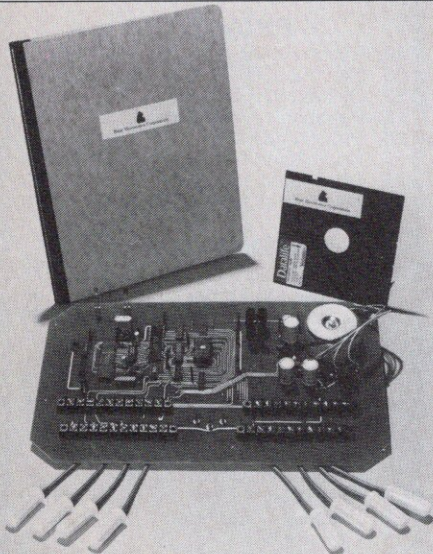
The SABRE Temperature Monitoring and Management System gathers data from eight temperature sensors.
