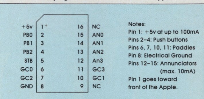
Figure 5: Connection of devices into the Apple's game I/O socket
