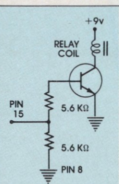
Figure 2: Annunciator output switches an NPN transistor, and the transistor controls a relay.
