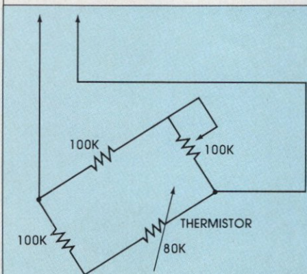
Figure 1: Fine-tuning with a Wheatstone Bridge
